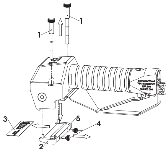
Fig. 6: Blade changing
