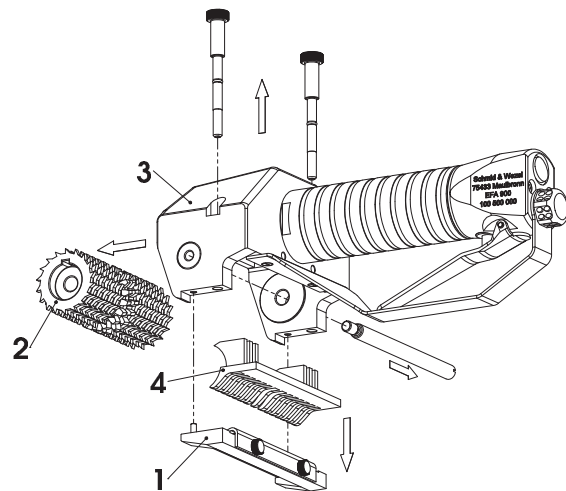
Fig. 8: Removing the cleaning claw
