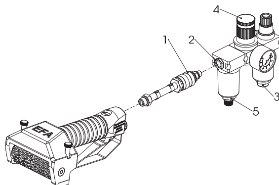
Fig. 1: Connecting to the air supply duct
