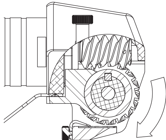
Fig. 5: Sectional drawing through the roller, direction of teeth
